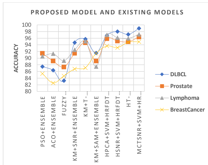
Figure 2: Comparison of proposed model to existing models on average feature selection
